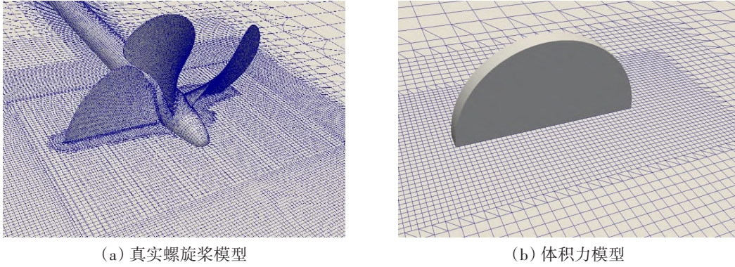
图7 KP505螺旋桨敞水试验模拟网格 Fig.7 Grids of KP505 propeller open-water test simulation
