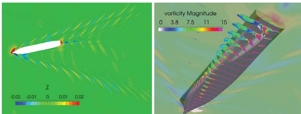
Figure 1: Numerical results of wave pattern and vortex of the container ship with drift angle \beta = 12^{\circ}
