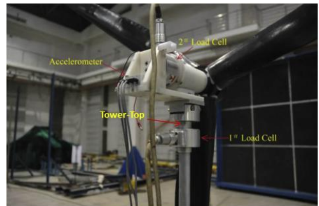
Fig. 21. Tower-top structure and sensors.
