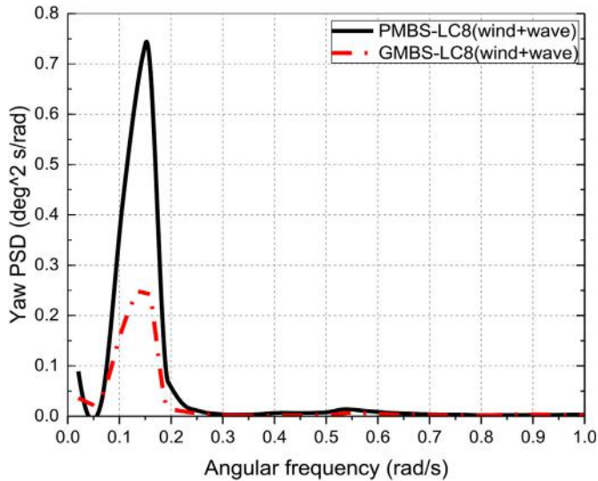
Fig. 19. Comparison of yaw motion in LC8.
