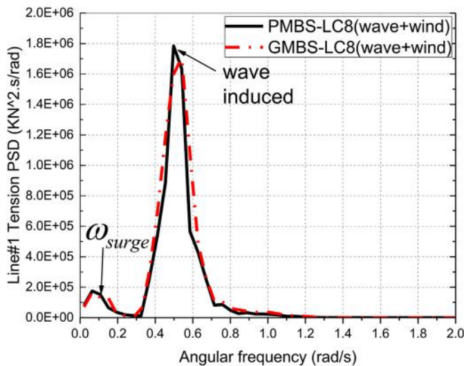
Fig. 28. Tension of the line#1 in LC8.
