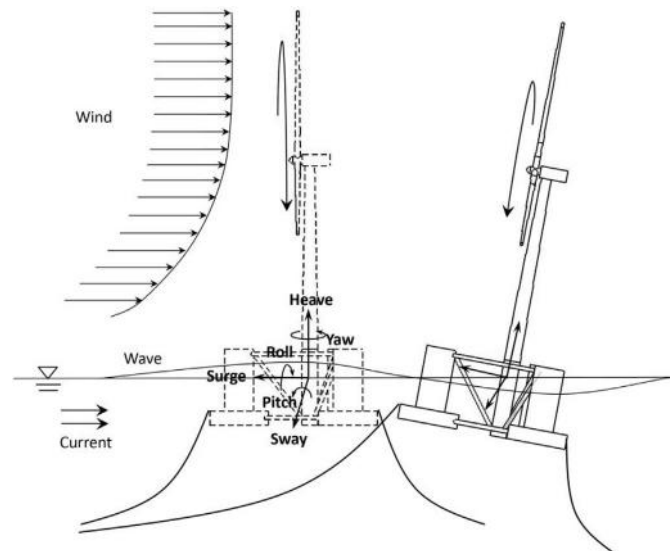
Fig. 10. 6-DOF motion of a semi-submersible FOWT.
