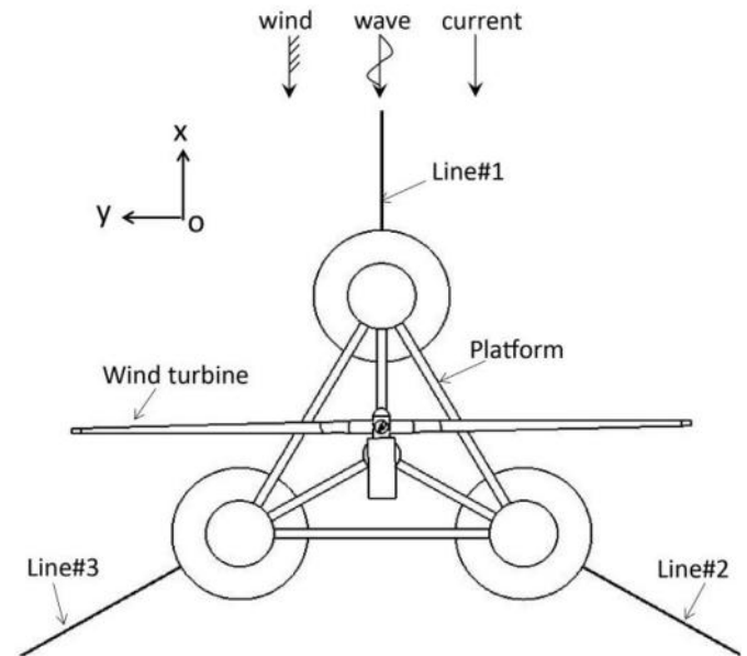
Fig. 26. Construction of the mooring-lines system.
