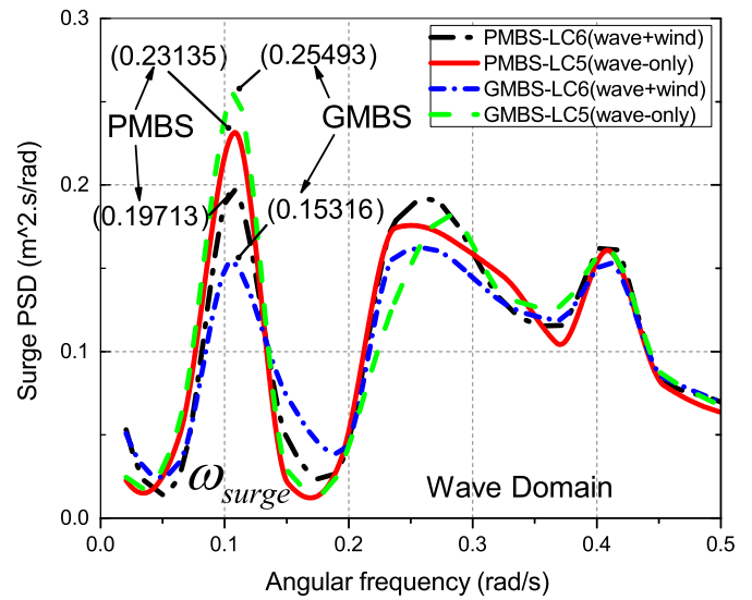
Fig. 16. Comparison of surge motion in LC5 and LC6.
