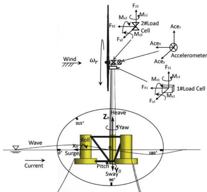
Fig. 5. Reference coordinates and sensors of the experimental model.
