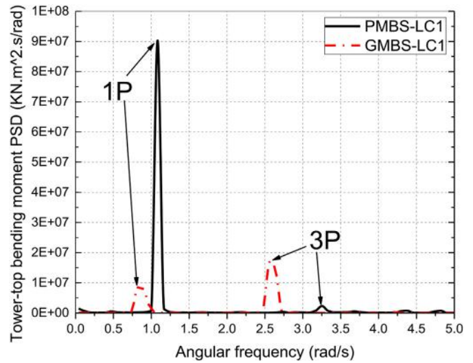
Fig. 25. Comparison of the tower-top bending moment in LC1.
