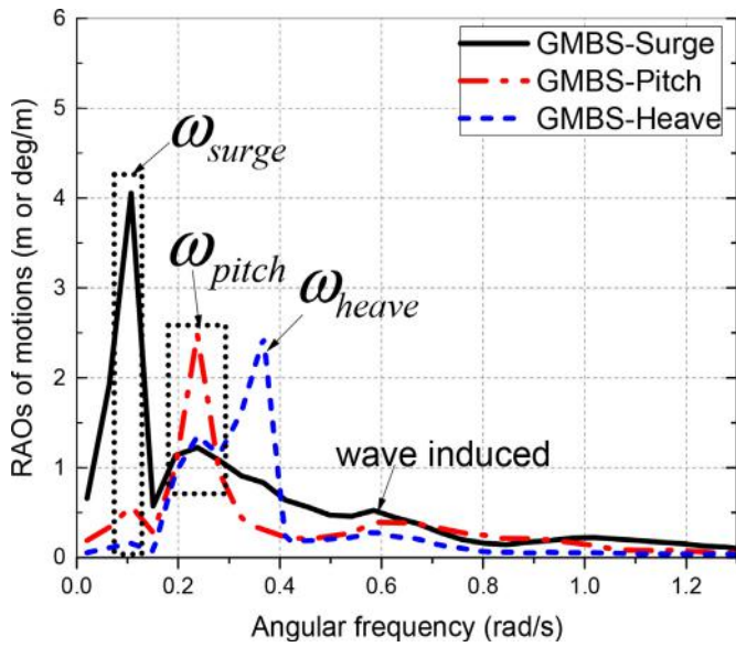
Fig. 14. RAOs of surge, pitch and heave motion of the GMBS model in LC5.
