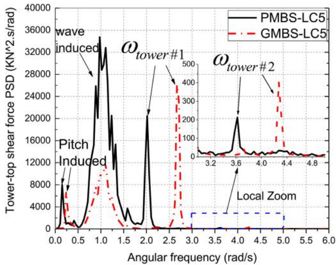
Fig. 22. Comparison of the tower-top shear forces in LC5.
