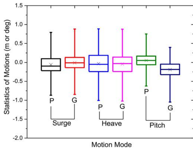
Fig. 12. Comparison of wave-induced motions in LC5.
