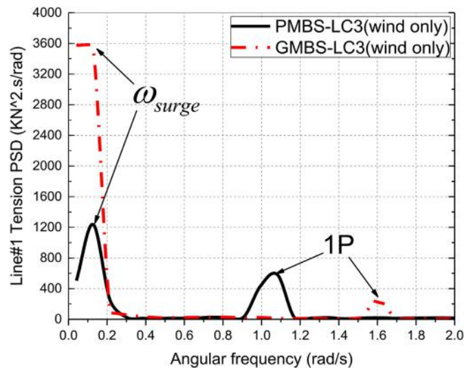
Fig. 29. Tension of the line#1 in LC3.
