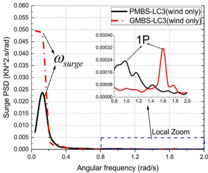
Fig. 30. Surge motion PSD in LC3.
