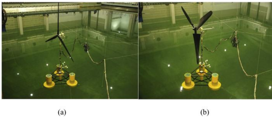
Fig. 3. Comparison of (a) geometrically matched blade model and (b) performance-matched blade model.
