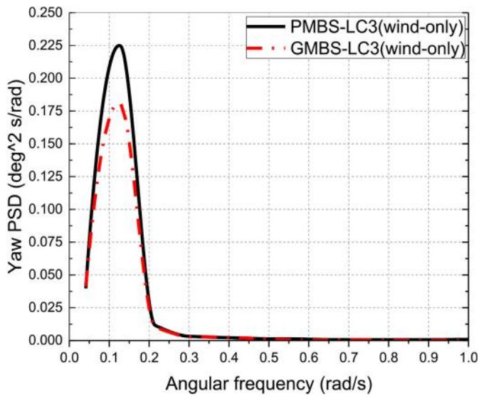
Fig. 18. Comparison of yaw motion in LC3.
