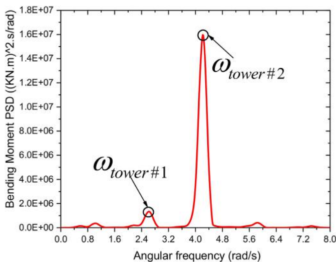
Fig. 8. Tower eigenfrequencies.
