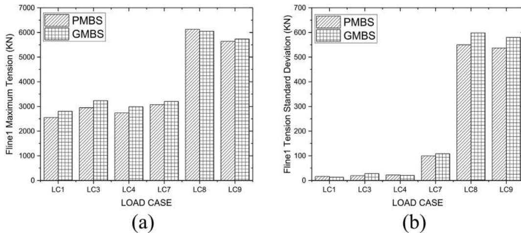
Fig. 27. Comparison of tension of the line#1: (a) maximum value. (b) standard deviation.
