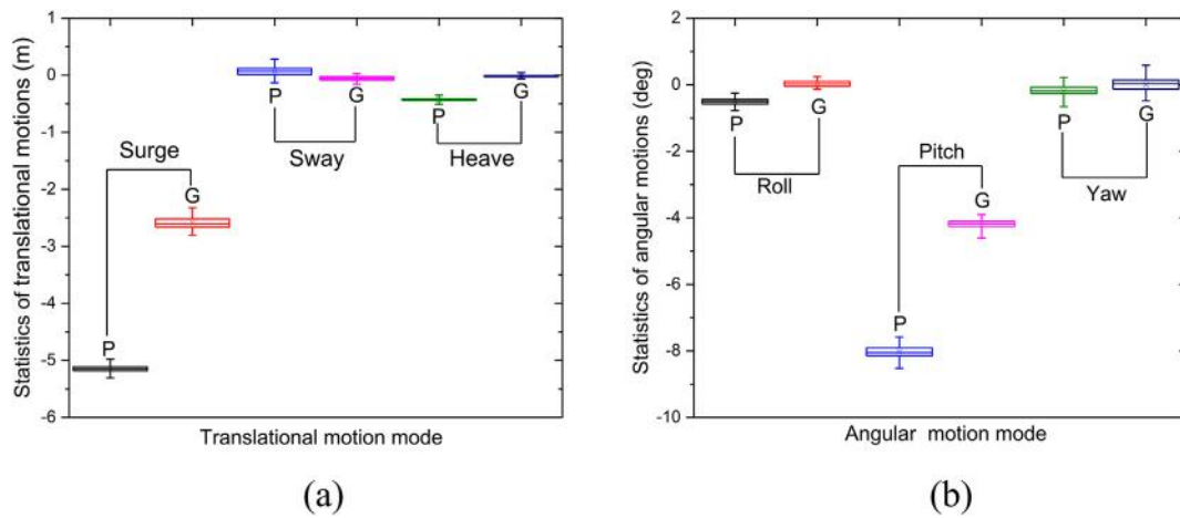
Fig. 11. Comparison of aero-induced motions in LC3.
