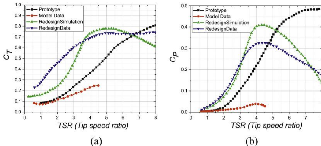
Fig. 1. Comparison of the aerodynamic coefficients (Fowler et al., 2013).
