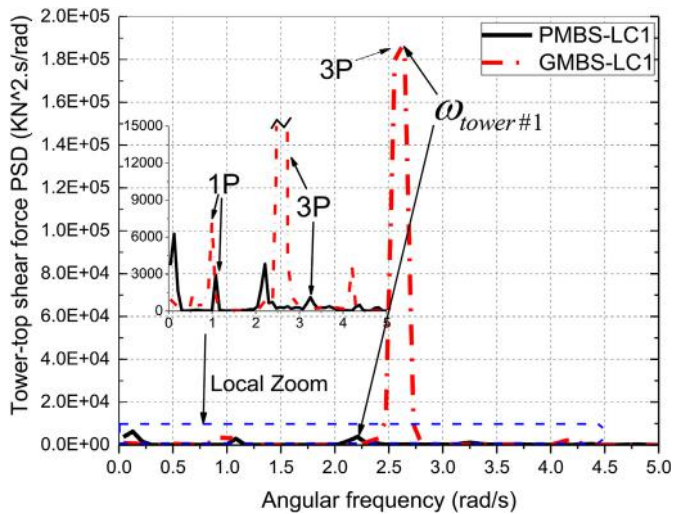
Fig. 23. Comparison of the tower-top shear forces in LC1.
