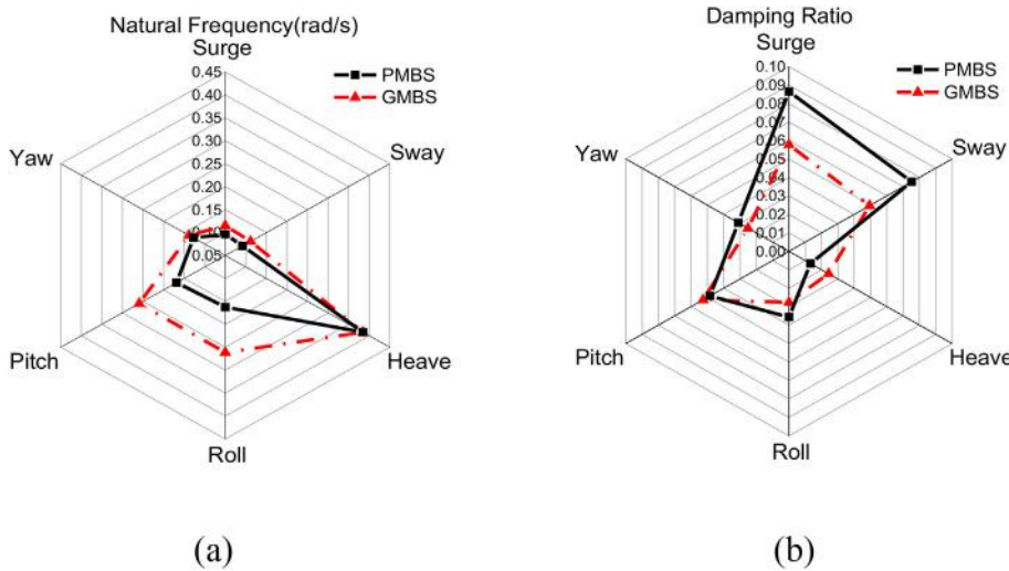
Fig. 9. Comparisons of (a) natural frequencies and (b) damping ratio.
