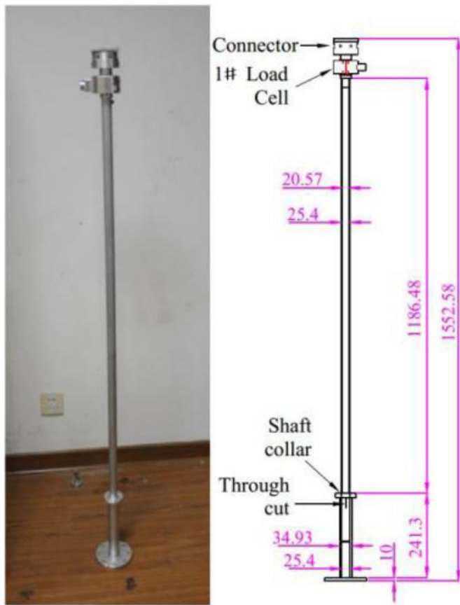
Fig. 7. Tower construction (Duan et al., 2016a).
