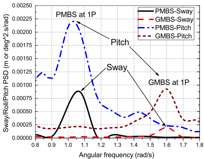
Fig. 31. Comparison of sway and pitch motion PSD in LC3.
