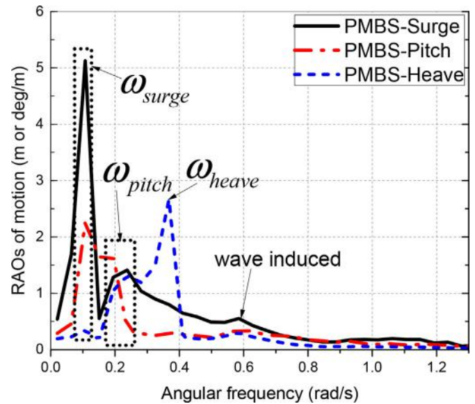
Fig. 13. RAOs of surge, pitch and heave motion of the PMBS model in LC5.
