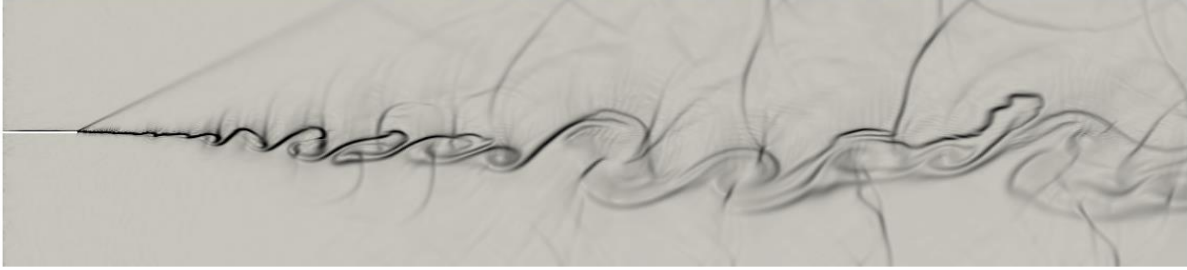
(a) Numerical schlieren contour of Case 1.
