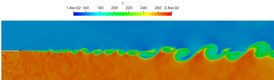
(c)Static temperature distribution contours of Case3.
